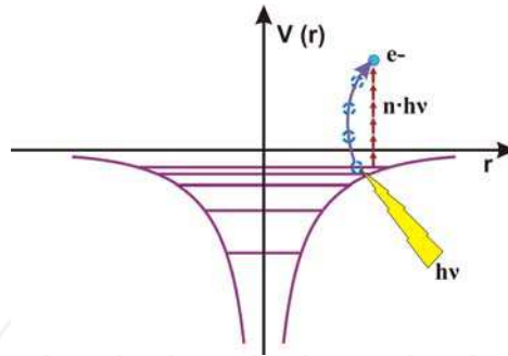
Fig. 5. Multiphoton ionization process: n-photons are absorbed. The total energy of absorbed photons ( n \cdot h\nu ; n - number of absorbed photons, h - Planck's constant, \nu - light frequency) exceeds ionization potential.
