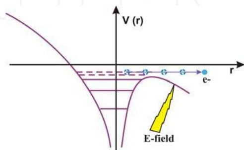
Fig. 4. In this case, the applied electric field is higher than the atomic field strength. The atomic potential barrier is suppressed and electrons from most-outer shells are liberated through above barrier ionization.
